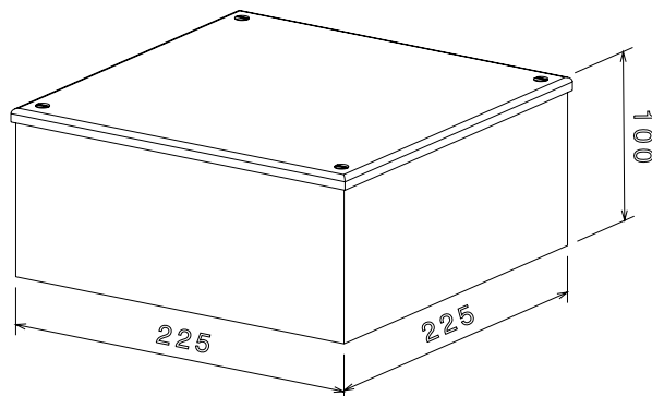
Isometric view
